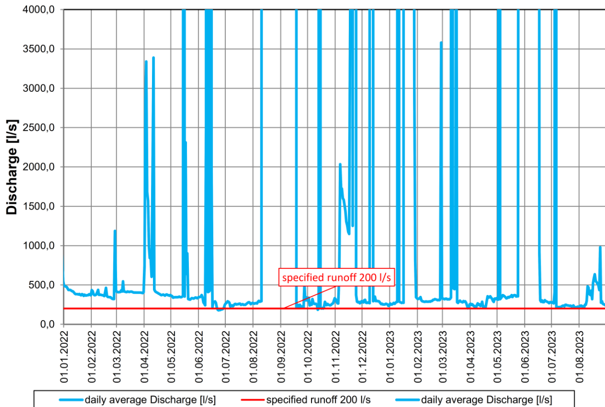
Diagram: Discharge at the intake
